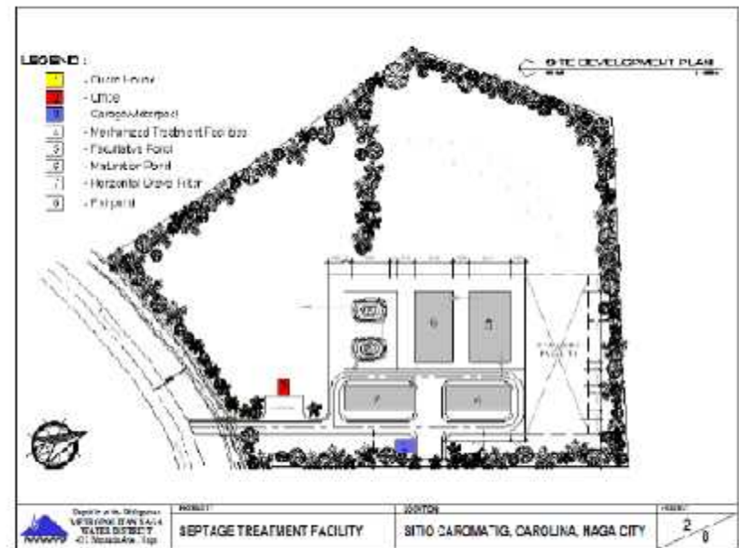
Figure 4.5: Layout of sludge treatment facility
